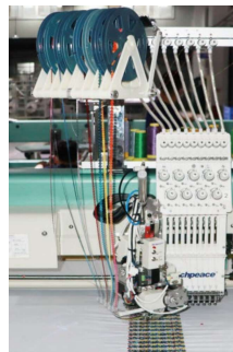
8-Sequin Device
