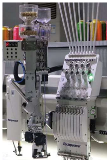
Multi-bead Device
